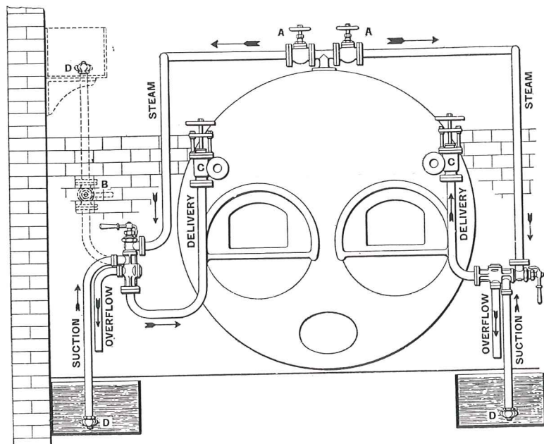
fig 1647...showing method of fixing the "One Movement" Injector
